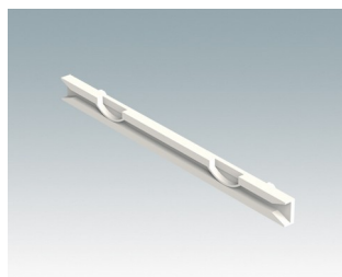
M6490010 Kartenführung, 102mm PA 6/6 (UL 94 V-0) Blank 101.6x7.5x3.5mm
